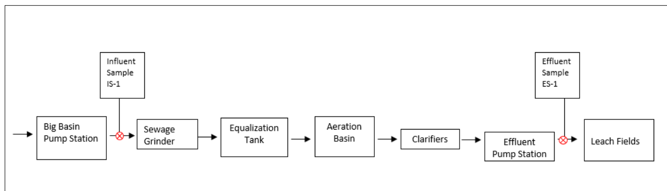
Figure 1. Process Flow Diagram with Sampling Locations
