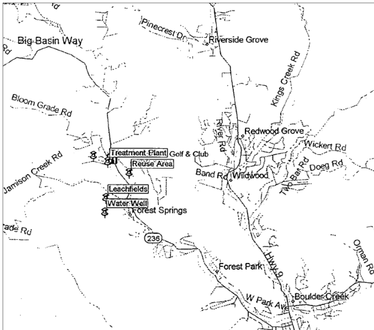
Figure 3. Dispersal System Layout
